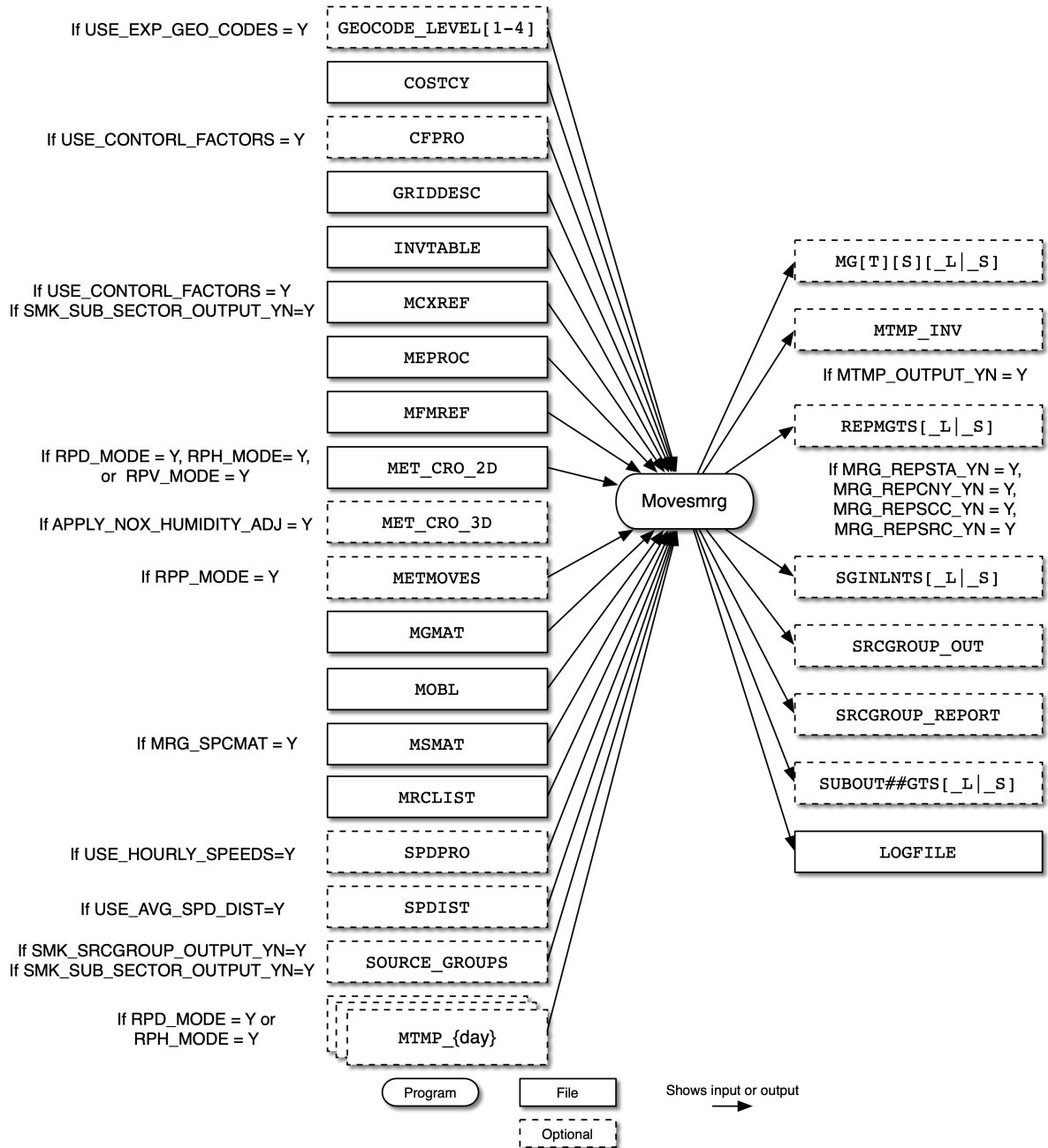
Figure 4.8, “ Movesmrg input and output files” [160] shows the input and output files for the Movesmrg program. The input files are the country, state, and county codes file (COSTCY), the grid description file (GRIDDESC), the inventory data table (INVTABLE), the representative county fuel month file (MFMREF), the list of emission process and associated pollutants file (MEPROC), the representative county cross-reference file (MCXREF), the list of emission factors files by representative county file (MRCLIST), the meteorology files (MET_CRO_2D), the gridding matrix from Grdmat (MGMAT), the inventory file output from Smkinven
