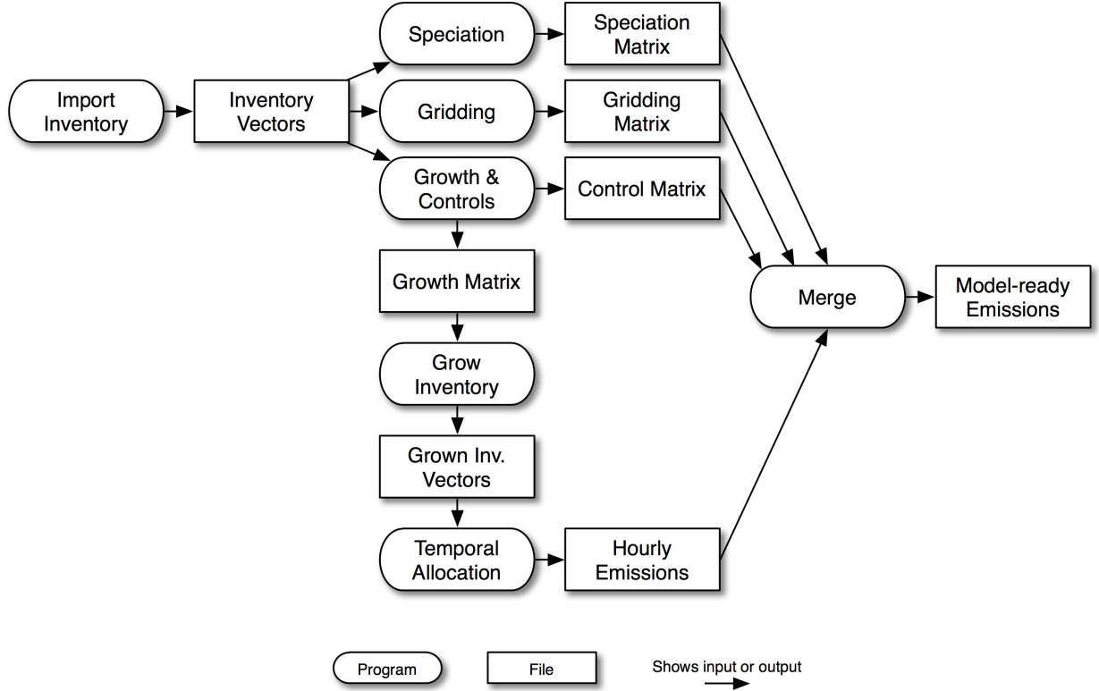
Figure 2.4. Parallel approach to emissions processing
