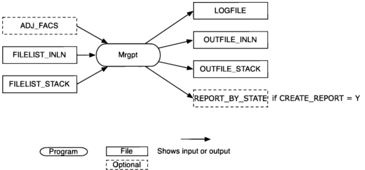
Figure 4.11. Mrgpt input and output files
