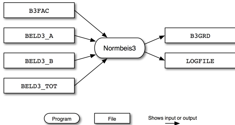
Figure 4.12. Normbeis3 input and output files for BEIS v3.14
