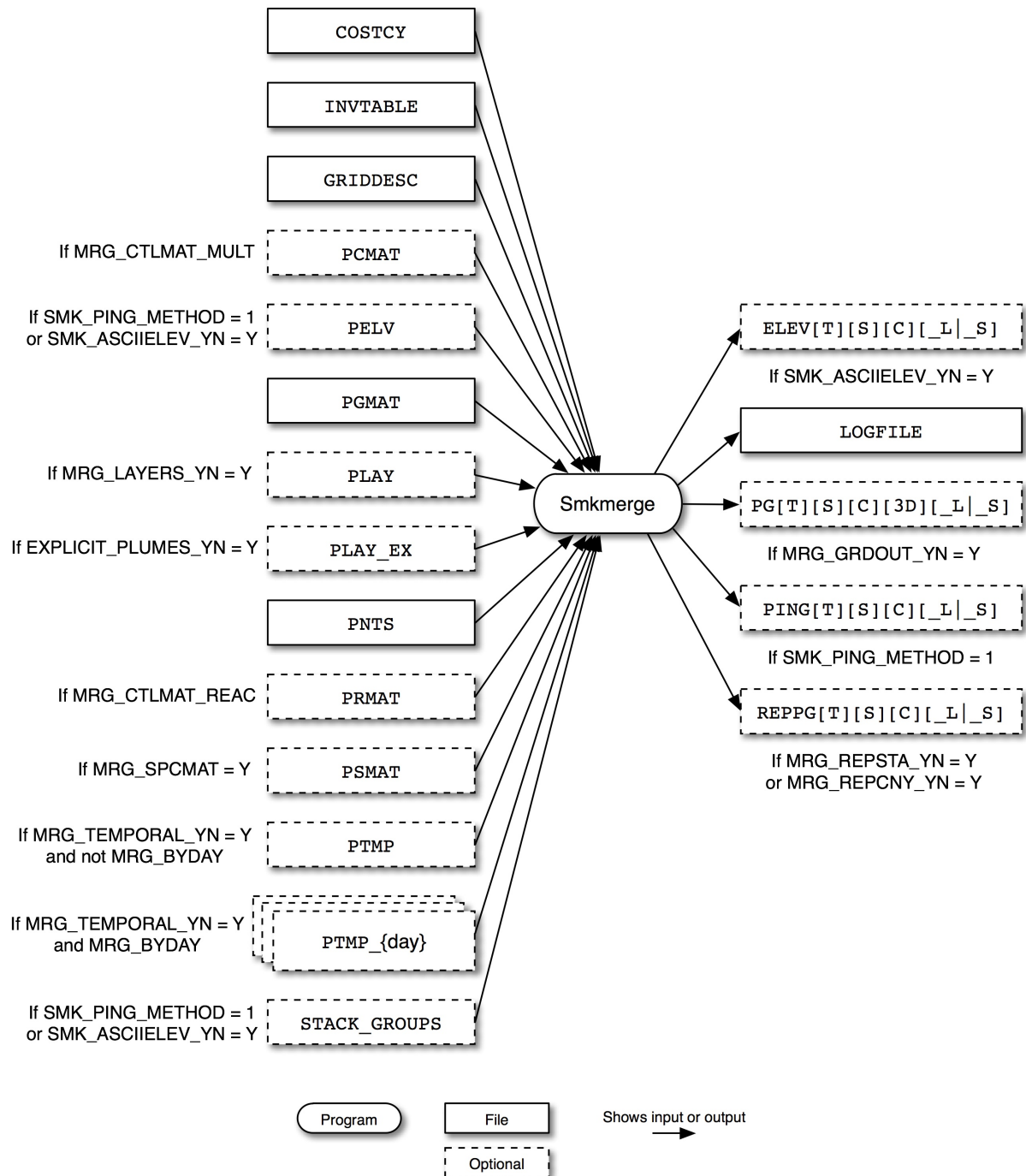
Figure 6.20. Smkmerge input and output files for point sources
