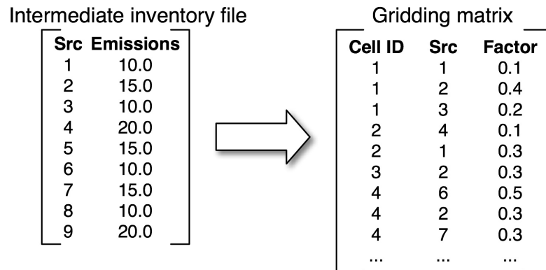
Figure 2.22. Relationship between inventory and gridding matrix
