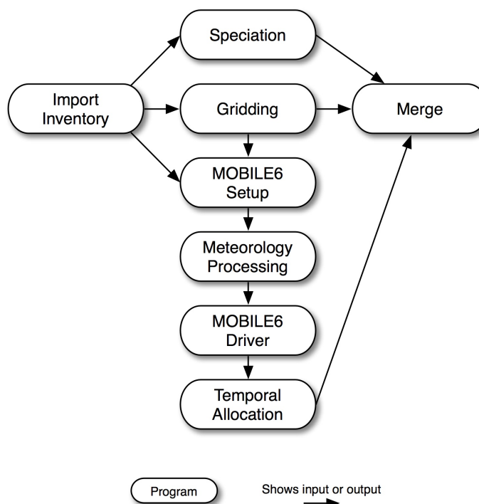
Figure 2.13. Base case mobile VMT approach processing steps
