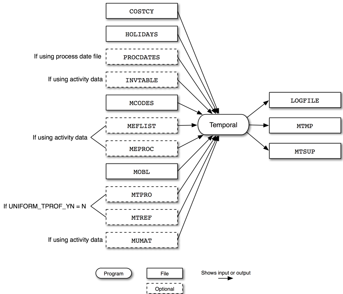
Figure 6.24. Temporal input and output files for mobile sources
