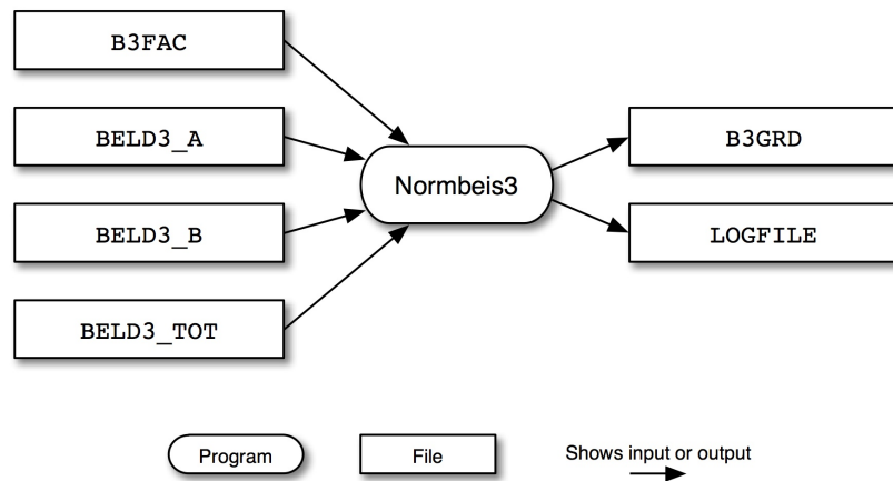
Figure 6.11. Normbeis3 input and output files
