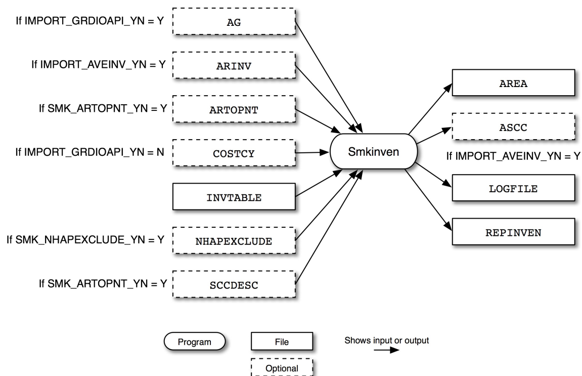
Figure 6.14. Smkinven input and output files for area sources
