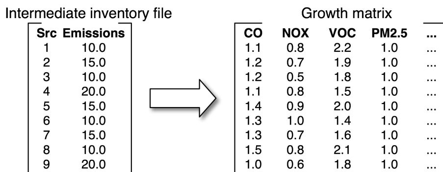
Figure 2.26. Relationship between inventory sources and growth matrix
