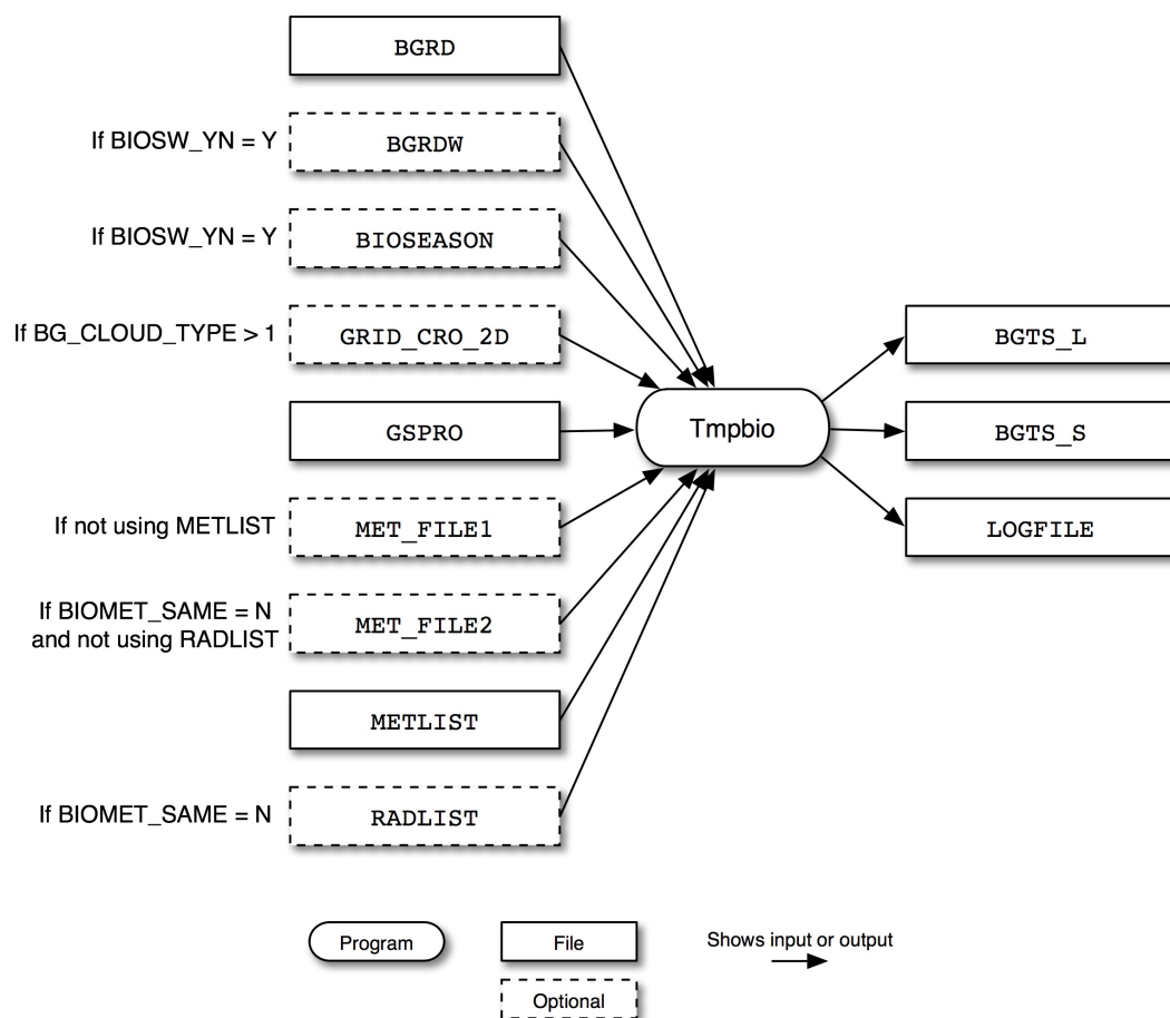
Figure 6.27. Tmpbio input and output files
