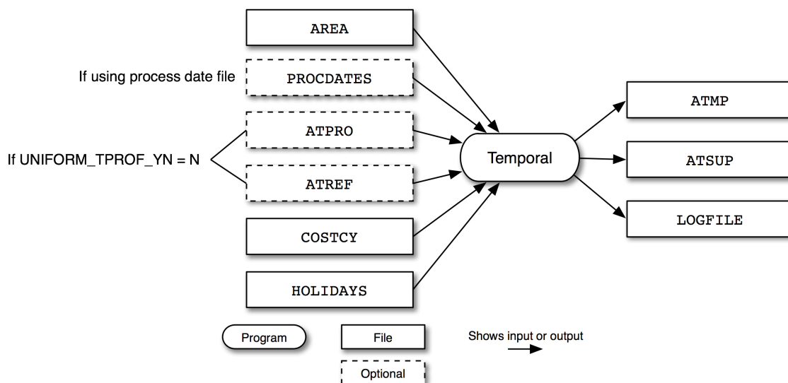
Figure 6.23. Temporal input and output files for area sources
