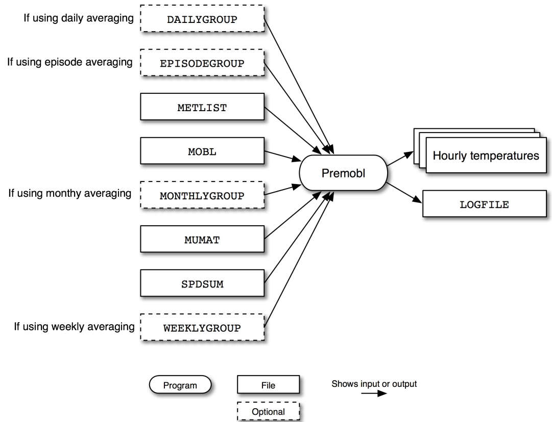
Figure 6.12. Premobl input and output files
