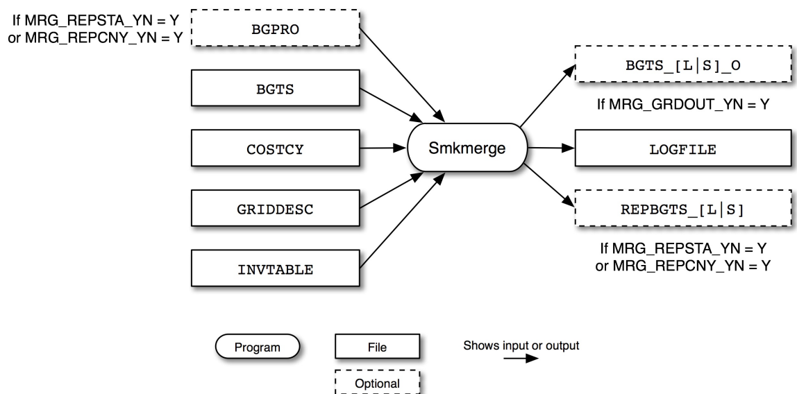
Figure 6.18. Smkmerge input and output files for biogenic sources
