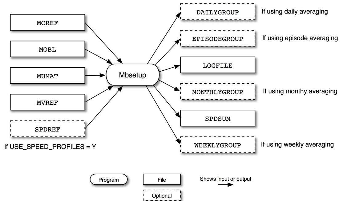
Figure 6.8. Mbsetup input and output files
