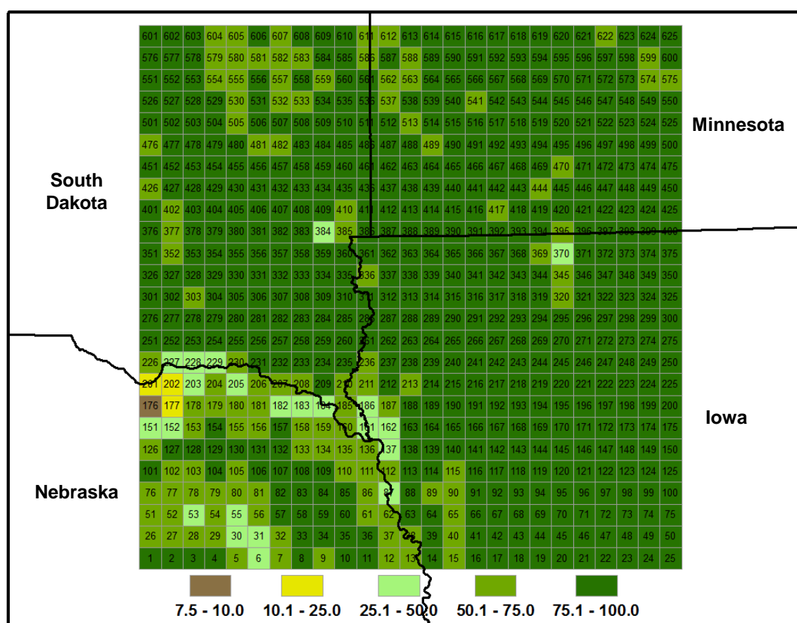
Figure 7. FEST-C test case 12-km domain in the northern Central Plains of the U.S. Each grid cell has an identification number (GRIDID) associated with it, along with a color that indicates crop coverage percentage. The cells are numbered from 1 for the lower left corner cell to 625 (25 rows × 25 columns) for the upper right corner cell of the domain.
